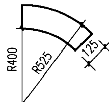
C30预制混凝土砌块大样
