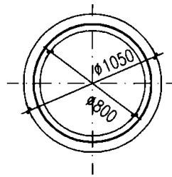
预制井筒大样
