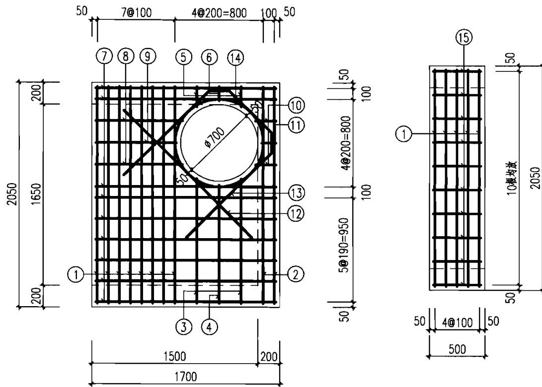
板3(a)
